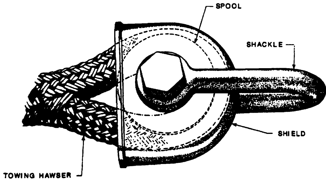
Figure 582-10-2 Rope Connector. (Nylite Spool, Shield and Shackle)
